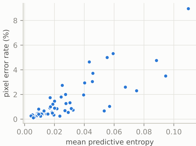
Per-image: entropy vs error ( r = 0.83 )
